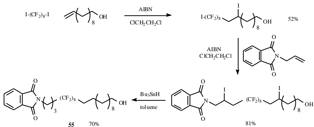
Fig. (31). The synthesis of N-protected semi-fluorinated alcohol ( 55 ).
