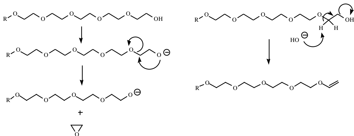
Fig. (3). The side reactions observed for penta and hexa ethylene glycol terminated compounds.
