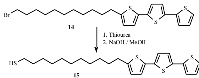
Fig. (11). The Synthesis of 11-[2,2';5',2'']terthiophen-5-yl-undecane-1-thiol ( 15 ).
