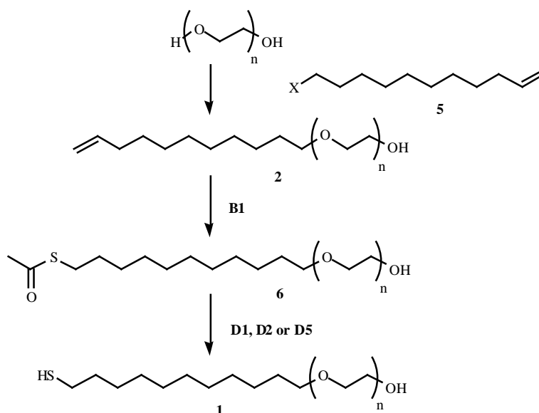
Fig. (6). The synthetic scheme for preparation of ethylene glycol terminated thiols.
