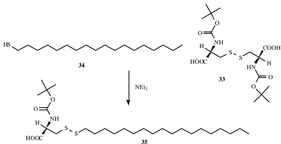
Fig. (20). An example of disulfide exchange for synthesis of unsymmetrical disulfide (35).
