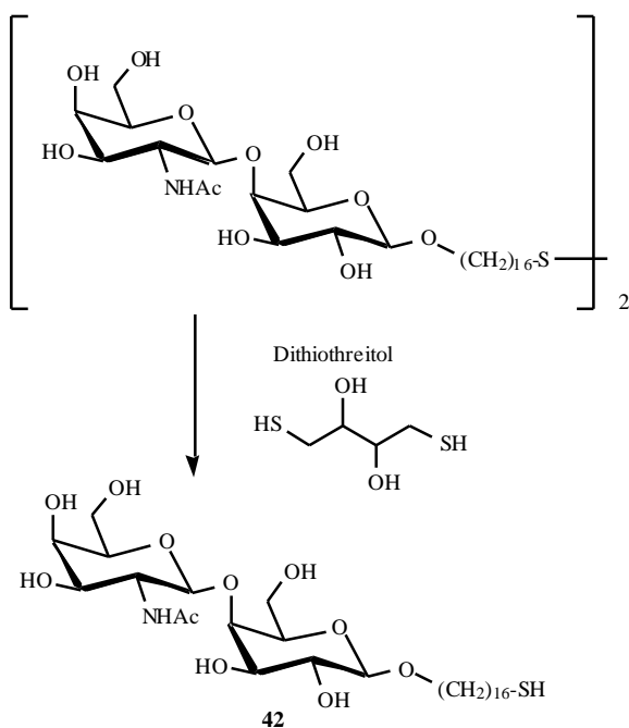
Fig. (24). The synthesis of carbohydrate terminated thiol ( 42 ).
