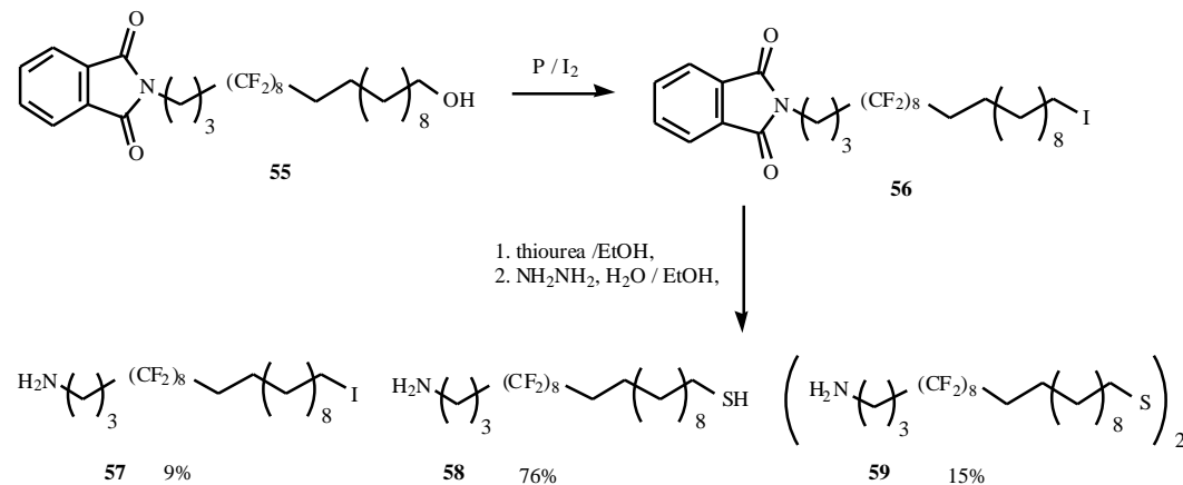
Fig. (32). The synthesis of alkanethiol ( 58 ) from iodide ( 56 ) and thiourea.
