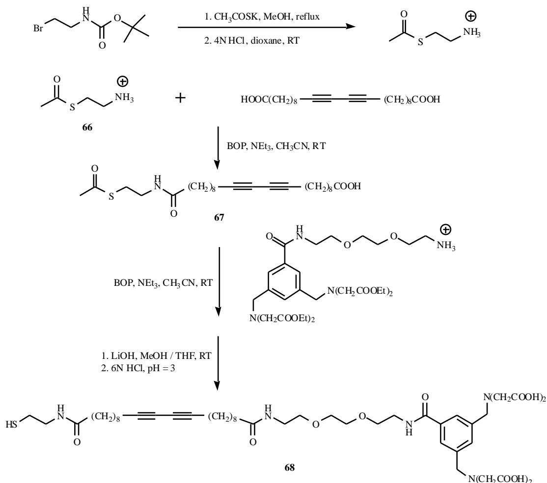
Fig. (35). The synthesis of a metal-chelating thiol (68).
