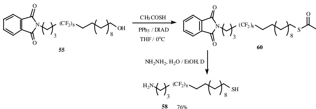
Fig. (33). The synthesis of amino-terminated semi-fluorinated long-chain alkanethiol ( 58 ).
