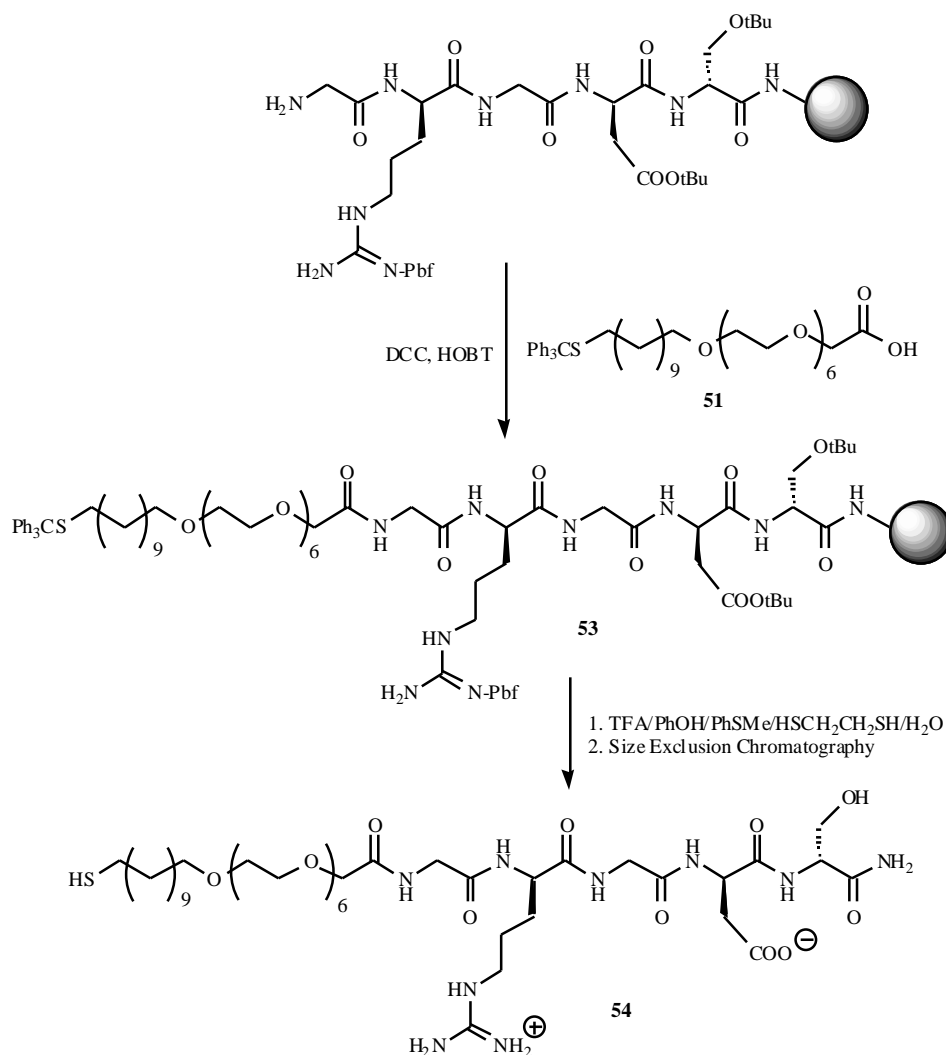
Fig. (30). The synthesis of pentapeptide terminated thiol (54).
