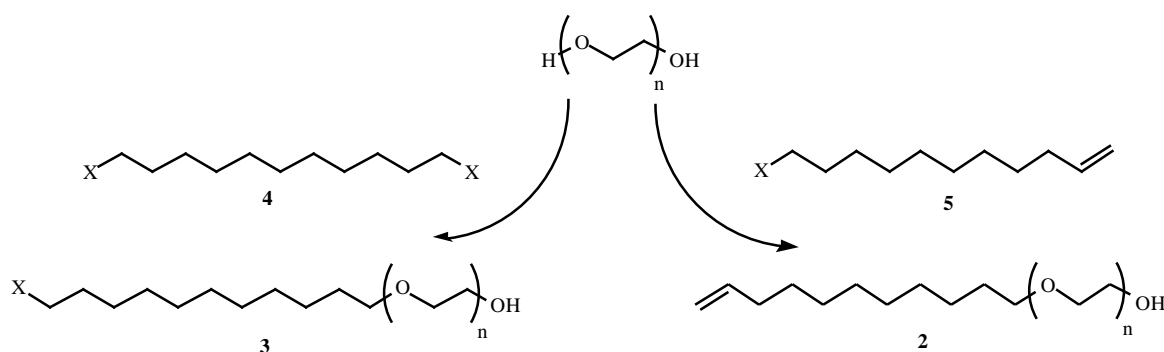
Fig. (5). The preparation of intermediates (2) and (3).
