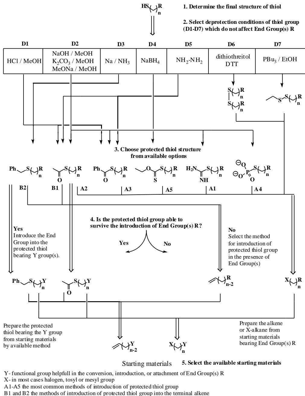
Scheme 1. Retrosynthesis of Functionalized Thiols
