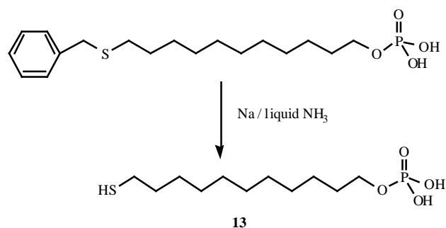
Fig. (10). The synthesis for phosphoric acid terminated thiol (13).
