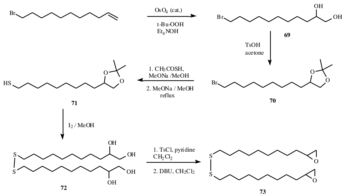
Fig. (36). The synthesis of epoxy-terminated dialkyl disulfides (73).
