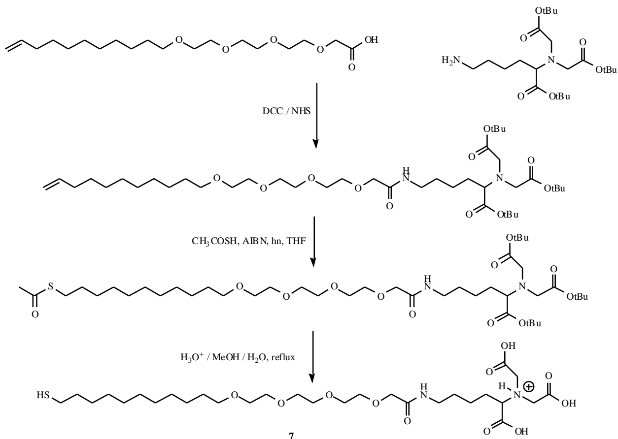
Fig. (7). The synthesis of nitrilotriacetic acid (NTA)-terminated alkanethiol (7).
