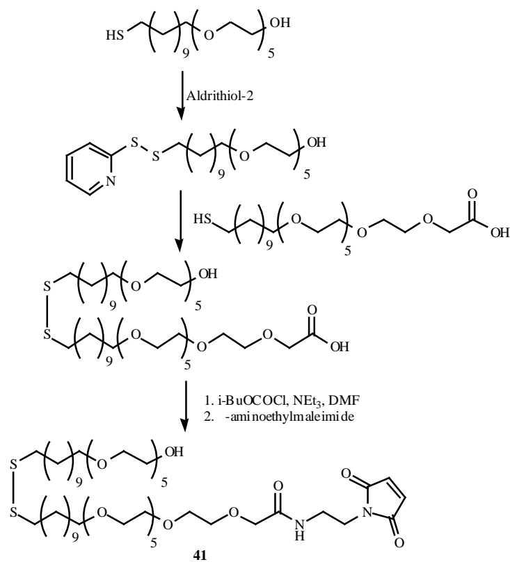
Fig. (23). The synthesis of an unsymmetrical disulfide (41).
