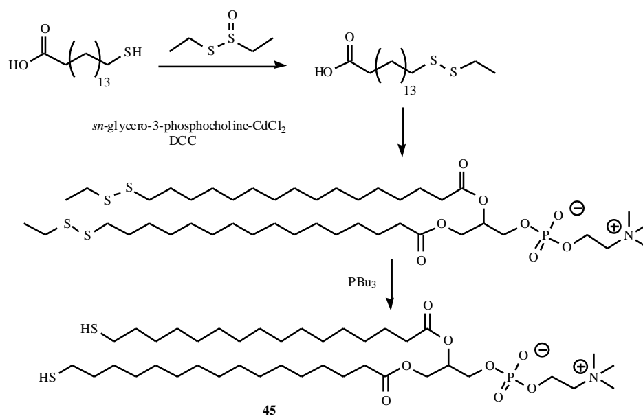
Fig. (26). The synthesis of glycero-3-phosphocholine terminated thiol ( 45 ).
