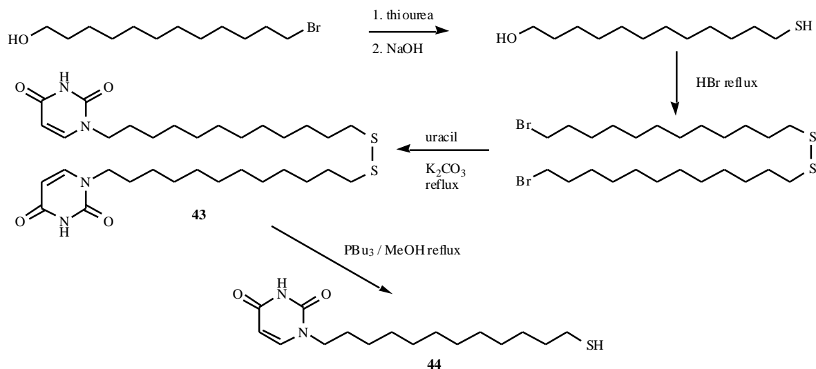
Fig. (25). The preparation of uracil terminated thiol ( 44 ).
