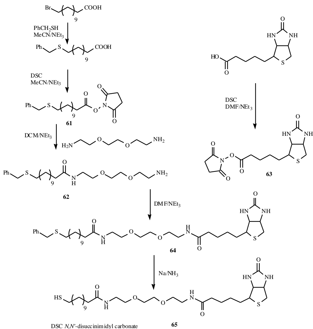
Fig. (34). The synthesis of biotinylated thiol ( 65 ).
