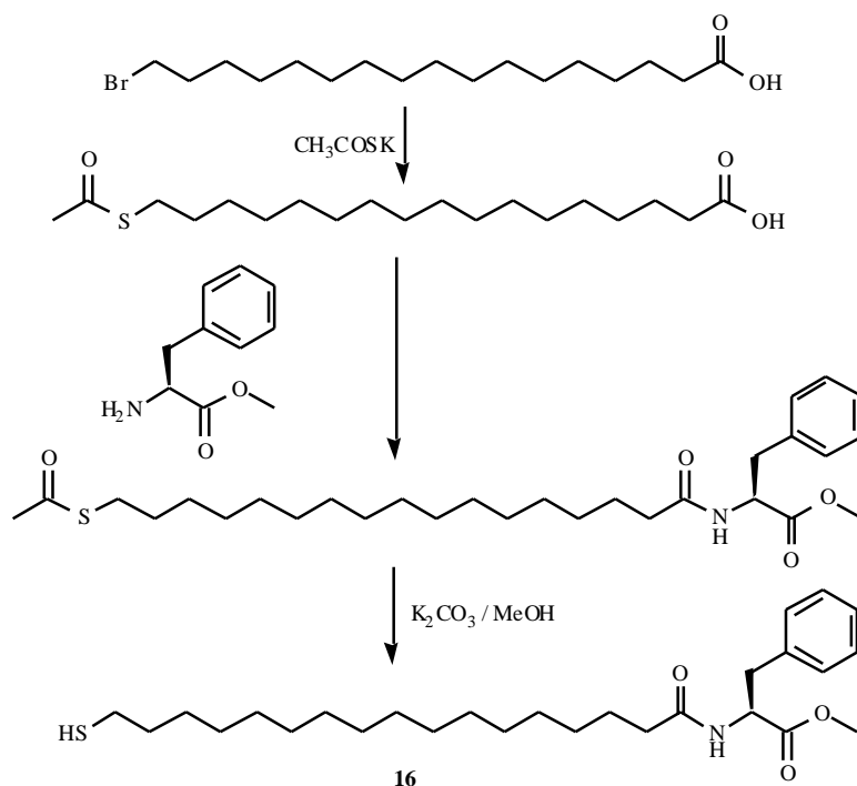
Fig. (12). The synthesis of N-( \alpha -thiol-heptadecanoyl)-phenylalanine methyl ester ( 16 ).
