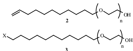
Fig. (4). The structure of the intermediates (2) and (3).
