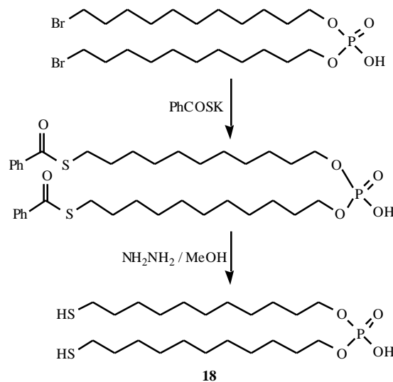
Fig. (14). The synthesis of bis(-mercaptoundecyl)phosphate ( 18 ).
