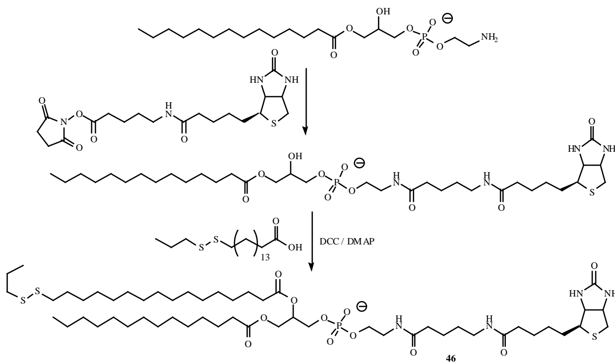
Fig. (27). The synthesis of dithio-phospholipids ( 46 ).
