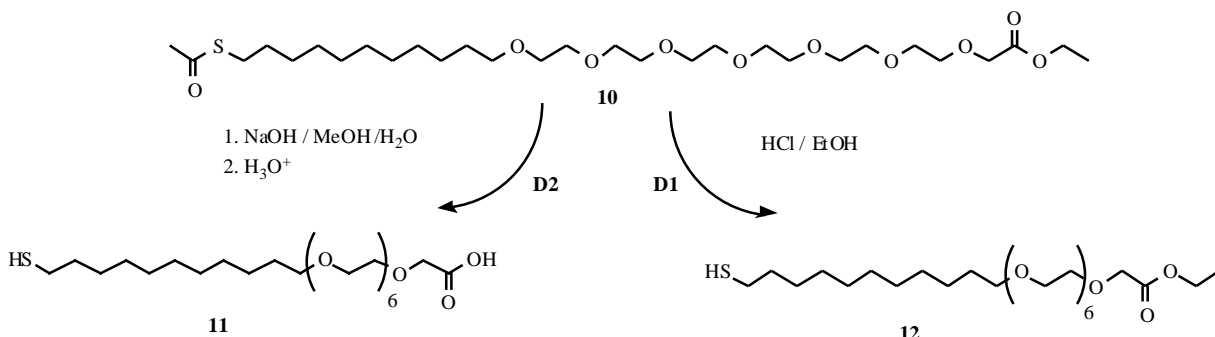
Fig. (9). The versatility of S-acetyl protective group.
