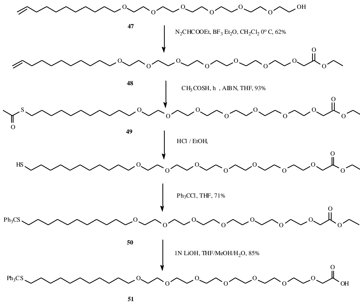
Fig. (28). The synthesis of (2-{2-[2-(2-[2-(11-tritylsulfanyl-undecyloxy)-ethoxy]-ethoxy)-ethoxy]-ethoxy}-ethoxy)-acetic acid ( 51 ).
