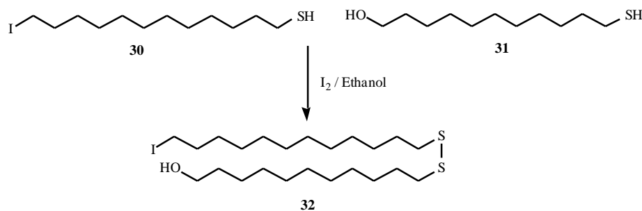
Fig. (19). The synthesis of 11-(12-iodododecylsulfanyloxy)undecan-1-ol ( 32 ).
