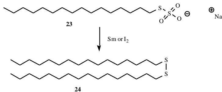
Fig. (17). The synthesis of dialkyldisulfides ( 24 ) from Bunte salt ( 23 ).
