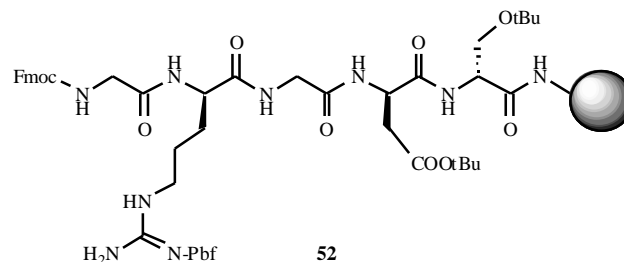
Fig. (29). The Fmoc-Gly-Arg-Gly-Asp-Ser pentapeptide ( 52 ) moiety on Fmoc-Rink amide MHBA polystyrene resin.
