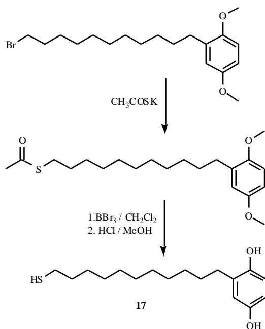
Fig. (13). The synthesis of 2-(11-mercaptoundecyl) hydroquinone ( 17 ).
