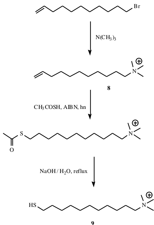
Fig. (8). The synthesis of ammonium terminated alkane thiol (9).
