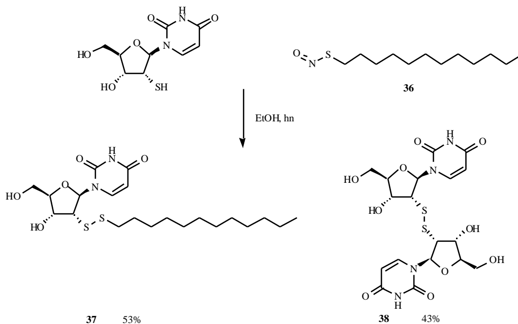
Fig. (21). The synthesis of 2'-Deoxyuridin-2'-yl-dodecyl disulfide (37).
