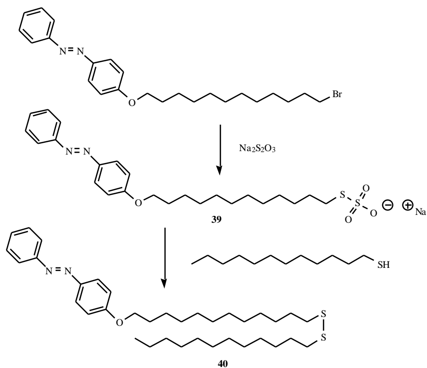
Fig. (22). The synthesis of unsymmetrical disulfide (40) from Bunte salt (39).
