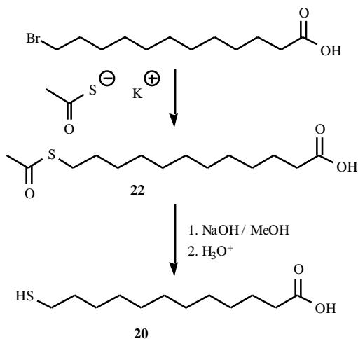
Fig. (16). The synthesis of 12-mercaptododecanoic acid ( 20 ) from potassium thioacetate.
