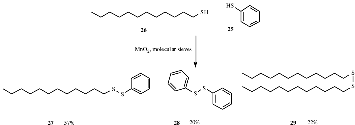
Fig. (18). The products distribution from Oxidation of mixture benzenethiol ( 25 ) and dodecane-1-thiol ( 26 ) with \text{MnO}_2 .
